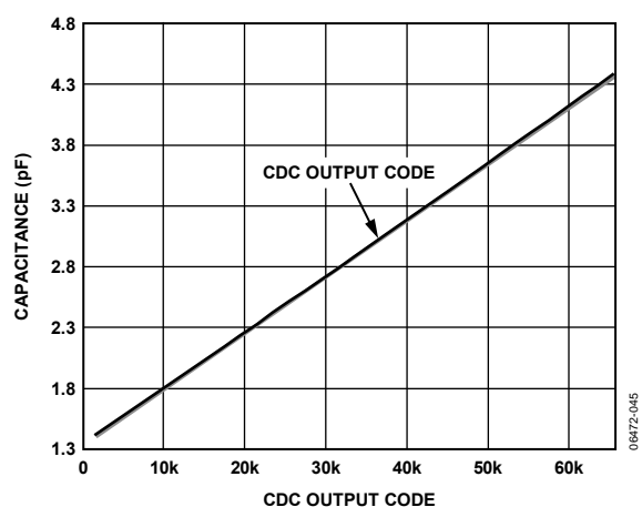
Figure 12. 3.3 V Linearity
