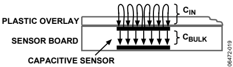
Figure 21. Capacitances Around the Sensor PCB
