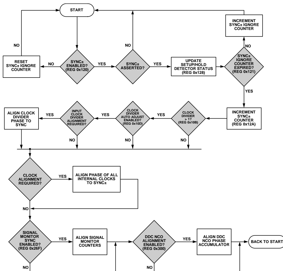
Figure 83. Multichip Synchronization
