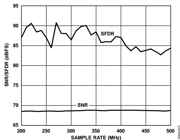
Figure 24. SNR/SFDR vs. Sample Rate ( f_S ); f_{IN} = 170.3 MHz;
