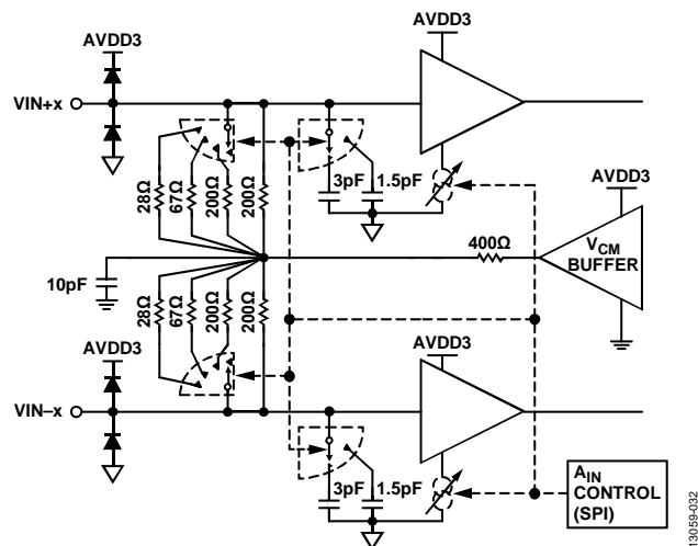
Figure 33. Analog Inputs
