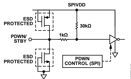
Figure 41. PDWN/STBY Input
