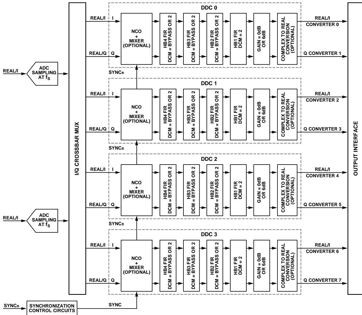
Figure 62. DDC Detailed Block Diagram
