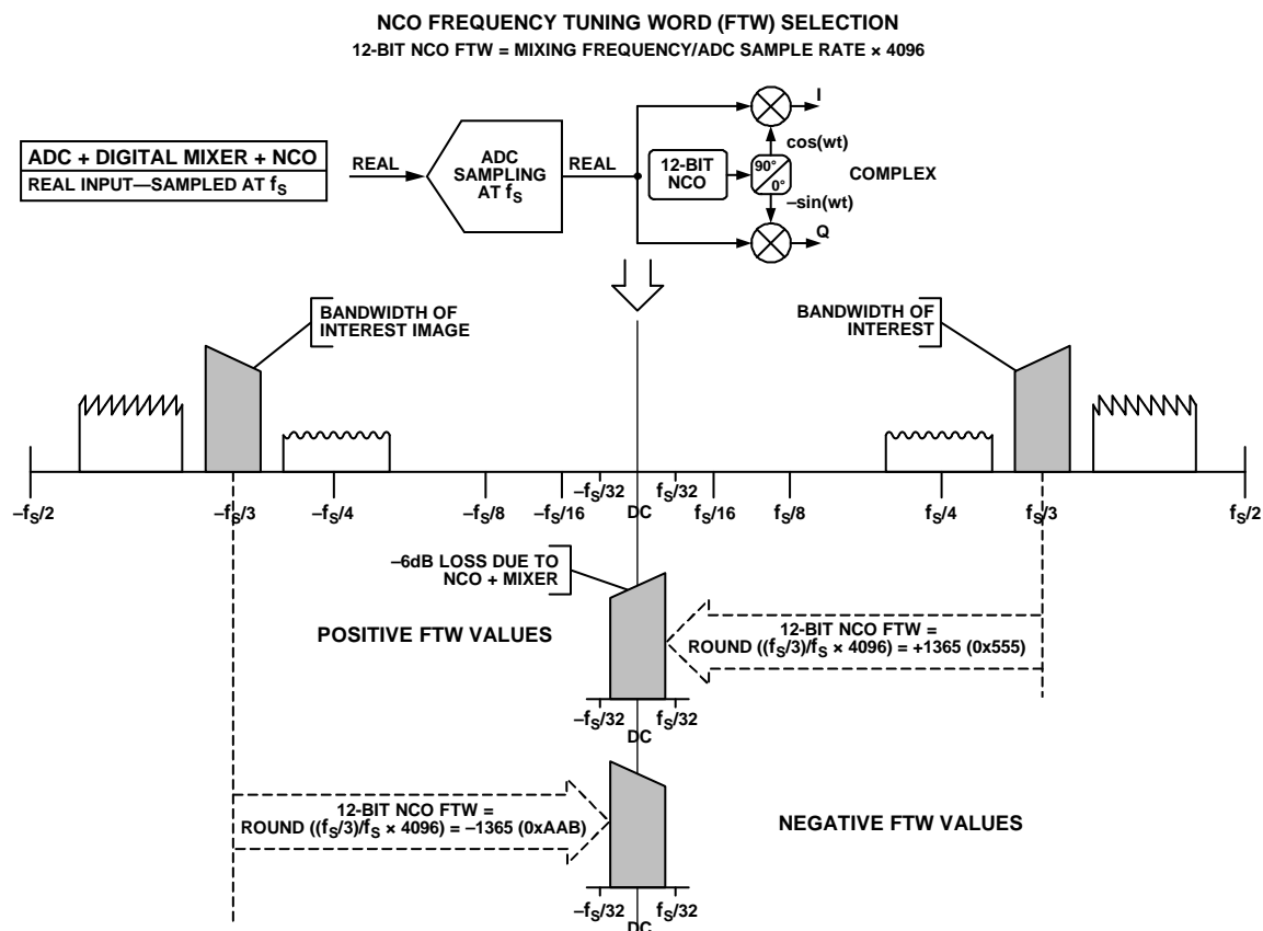
Figure 64. DDC NCO Frequency Tuning Word Selection—Real Inputs
