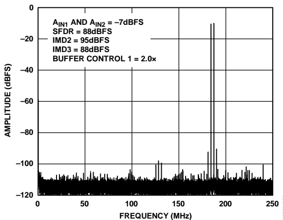
Figure 26. Two-Tone FFT; f_{IN1} = 184 MHz, f_{IN2} = 187 MHz
