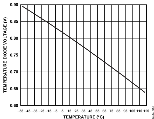
Figure 59. Temperature Diode Voltage vs. Temperature
