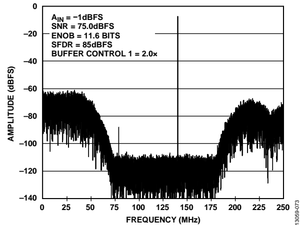
Figure 74. 21% BW Mode, Tuning Word = 26 ( f_3/4 Tuning)
