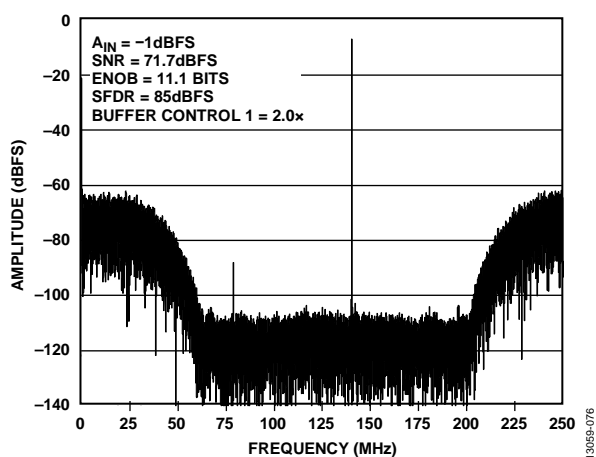
Figure 77. 28% BW Mode, Tuning Word = 19 ( f_s/4 Tuning)
