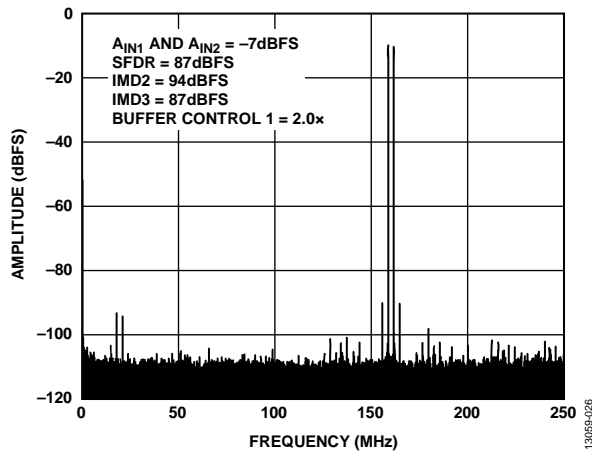
Figure 27. Two-Tone FFT; f_{IN1} = 338\text{ MHz} , f_{IN2} = 341\text{ MHz}
