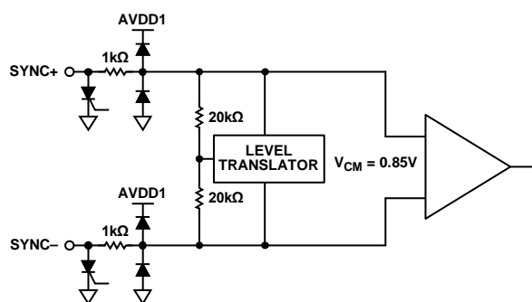
Figure 35. SYNC± Inputs
