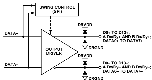
Figure 36. Digital Outputs
