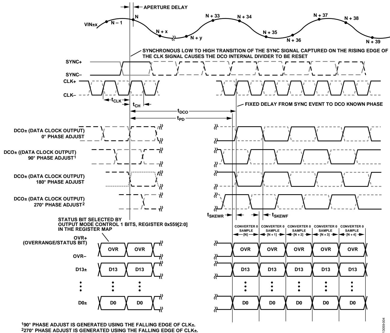
Figure 4. Parallel Interleaved Mode—One Virtual Converter
