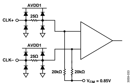
Figure 34. Clock Inputs
