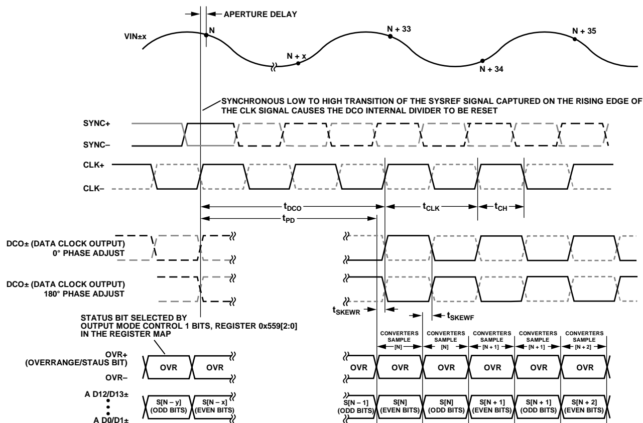
Figure 6. Channel Multiplexed (Even/Odd) Mode—One Virtual Converter
