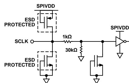
Figure 37. SCLK Inputs
