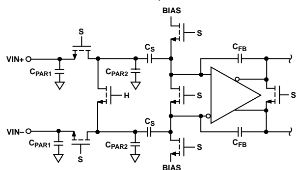
Figure 24. Switched-Capacitor Input
