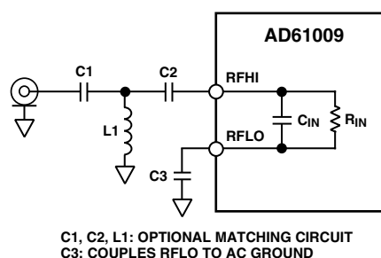
Figure 2. Mixer Port Modeled as a Parallel RC Network; an Optional Matching Network Is also Shown
