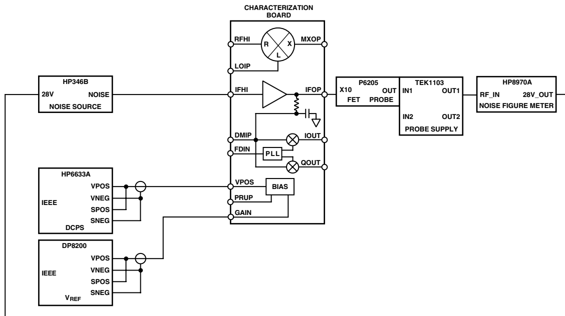
TPC 3. IF Amp Noise Figure Test Set
