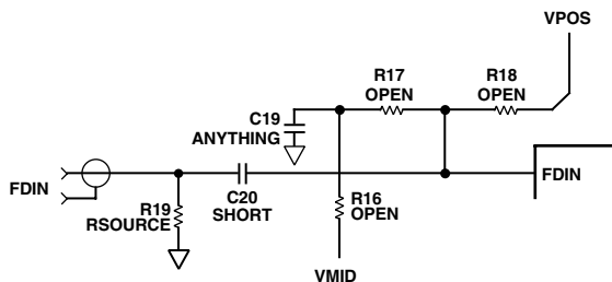
Figure 13. Evaluation Board
