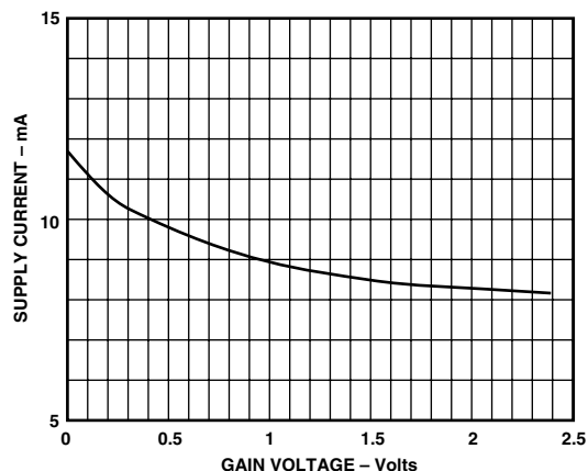
TPC 31. Power Supply Current vs. Gain Control Voltage, G_{REF} = 1.5\text{ V}
