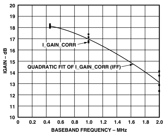
TPC 26. Demodulator Gain vs. Frequency
