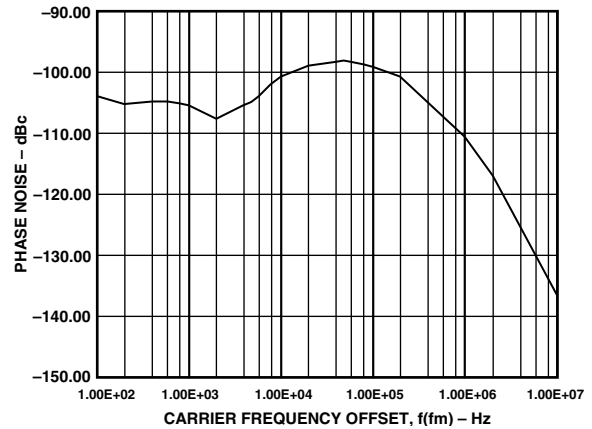
TPC 22. PLL Phase Noise L(F) vs. Frequency, V_{\text{POS}} = 3\text{ V} , C3 = 0.1\text{ }\mu\text{F} , \text{IF} = 10.7\text{ MHz}
