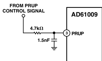
Figure 12. Proper Configuration of AD61009 PRUP Signal
