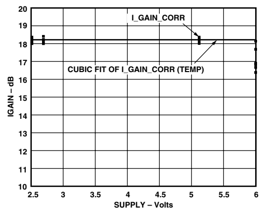
TPC 28. Demodulator Gain vs. Supply Voltage
