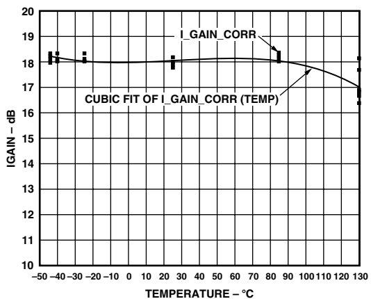
TPC 27. Demodulator Gain vs. Temperature
