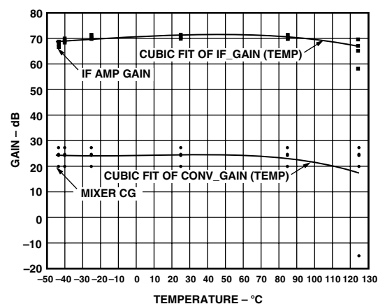
TPC 17. Mixer Conversion Gain and IF Amplifier Gain vs. Temperature, V_{\text{POS}} = 3\text{ V} , V_{\text{GAIN}} = 0.3\text{ V} , V_{\text{REF}} = 1.5\text{ V} , \text{IF} = 10.7\text{ MHz} , \text{RF} = 250\text{ MHz}
