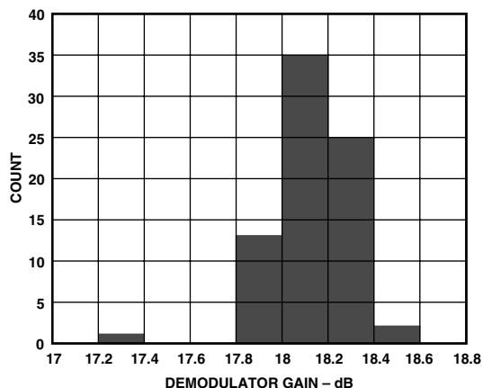
TPC 29. Demodulator Gain Histogram, T = 25^{\circ}\text{C} , V_{\text{POS}} = 3\text{ V} , \text{IF} = 10.7\text{ MHz}
