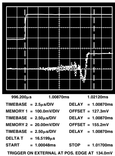
TPC 21. PLL Acquisition Time
