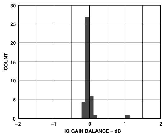
TPC 25. Demodulator Gain Balance, Histogram, T = 25^{\circ}\text{C} , V_{\text{POS}} = 3\text{ V} , \text{IF} = 10.7\text{ MHz}
