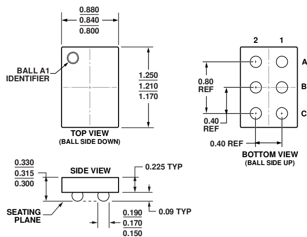
Figure 26. 6-Ball Wafer Level Chip Scale Package [WLCSP]
