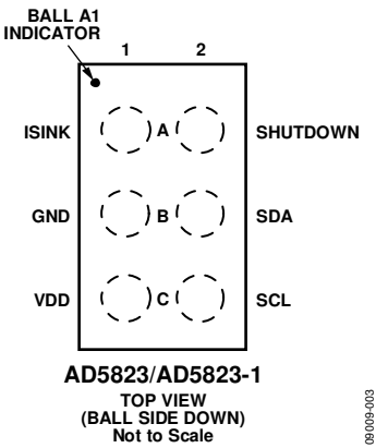
Figure 3. Pin Configuration
