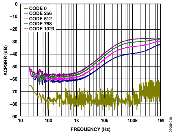
Figure 10. AC Power Supply Rejection Ratio, V_{DD} = 3\text{ V}
