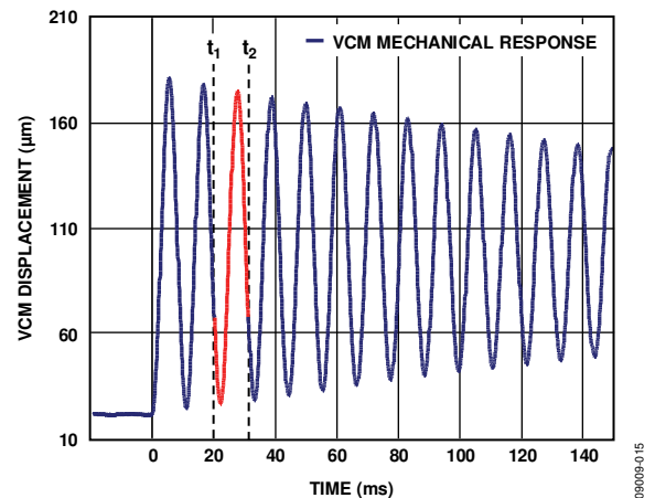
Figure 13. VCM Mechanical Response to a Step Current Input, t_{\text{RES}} = t_2 - t_1
