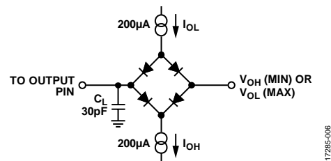
Figure 5. Load Circuit for the SDO Timing Diagram
