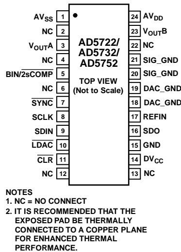
Figure 5. Pin Configuration
