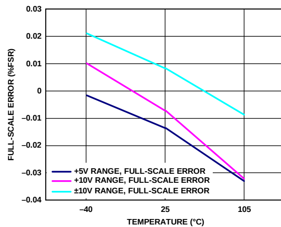
Figure 9. Full-Scale Error vs. Temperature
