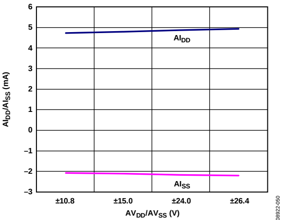
Figure 48. A_{I_{DD}}/A_{I_{SS}} vs. AV_{DD}/AV_{SS} , I_{OUT} = 0 mA
