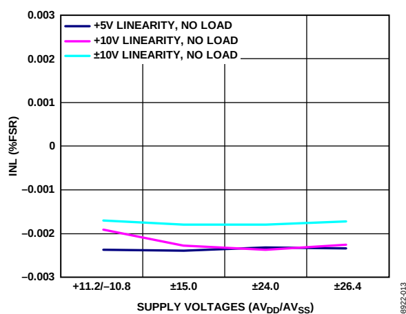
Figure 13. Integral Nonlinearity Error vs. Supply Voltage
