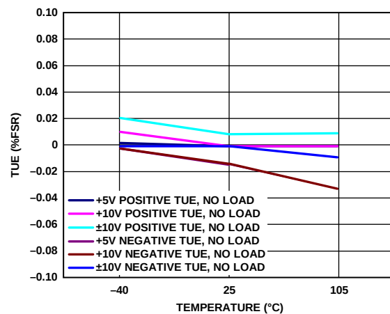
Figure 8. Total Unadjusted Error vs. Temperature
