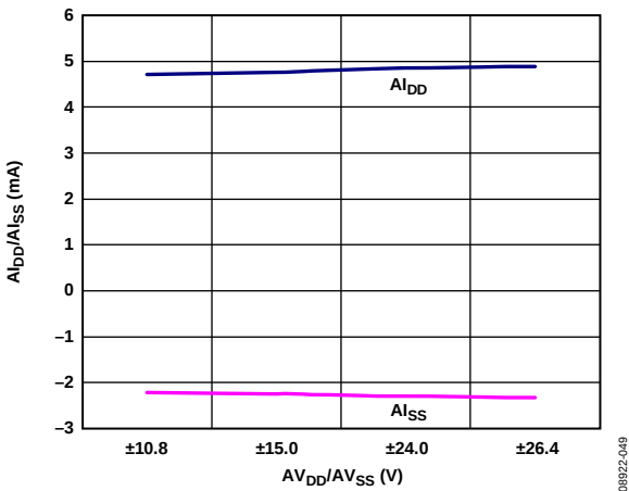
Figure 47. A_{I_{DD}}/A_{I_{SS}} vs. AV_{DD}/AV_{SS} , V_{OUT} = 0 V
