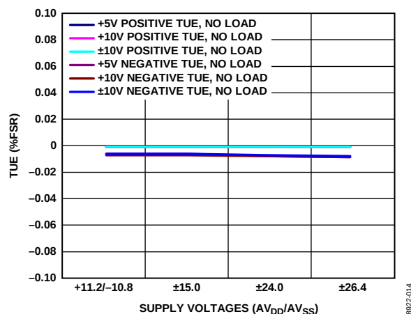
Figure 14. Total Unadjusted Error vs. Supply Voltages
