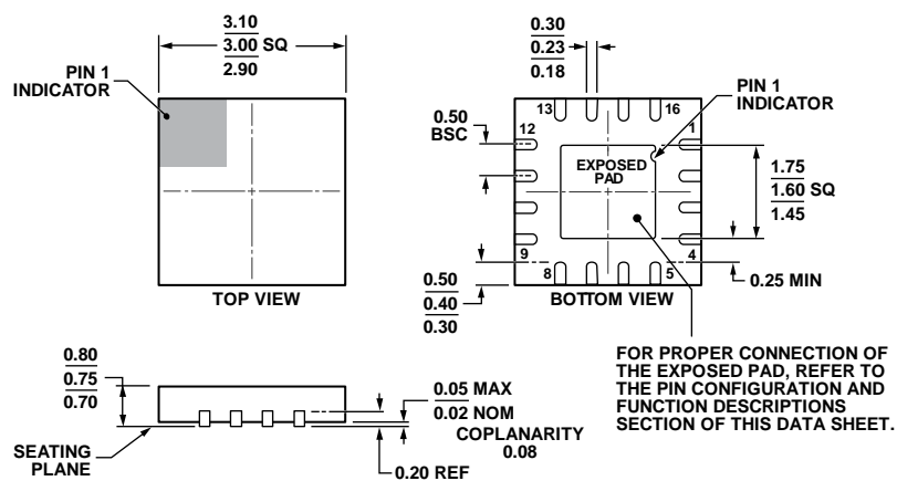
Figure 53. 16-Lead Lead Frame Chip Scale Package [LFCSP_WQ] 3 mm x 3 mm Body, Very Very Thin Quad (CP-16-22) Dimensions shown in millimeters
