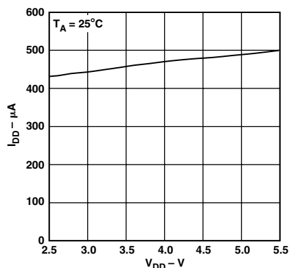
Figure 17. Supply Current vs. Supply Voltage
