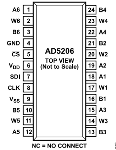
Figure 8. AD5206 SOIC/TSSOP Pin Configuration
