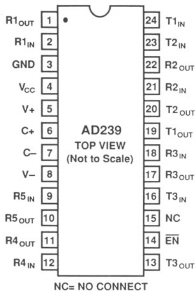
Figure 19. AD239 DIP/SOIC Pin Configuration
