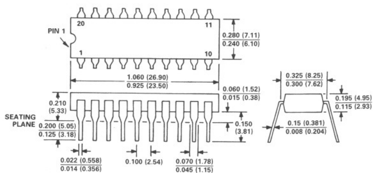
20-Lead Plastic DIP (N-20)
