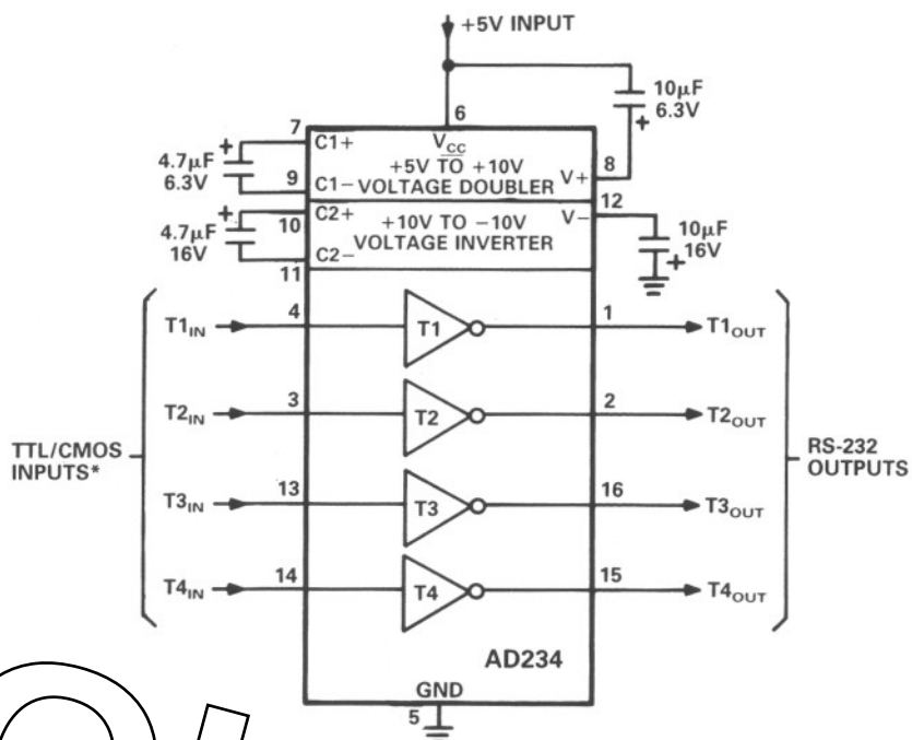
Figure 10. AD234 Typical Operating Circuit
