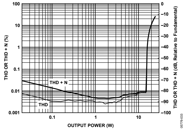
Figure 31. THD and THD + N vs. Output Power, 1 kHz Sine, 4 \Omega Load, PVDD = 20 V
