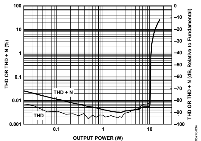
Figure 32. THD and THD + N vs. Output Power, 1 kHz Sine, 6 \Omega Load, PVDD = 20 V
