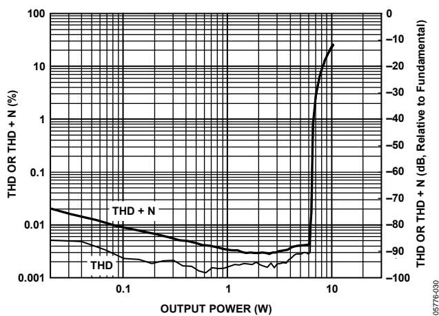
Figure 30. THD and THD + N vs. Output Power, 1 kHz Sine, 8 \Omega Load, PVDD = 18 V
