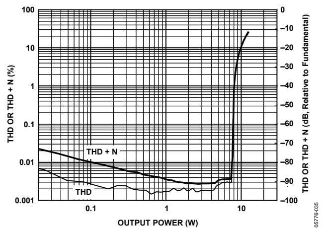
Figure 33. THD and THD + N vs. Output Power, 1 kHz Sine, 8 \Omega Load, PVDD = 20 V
