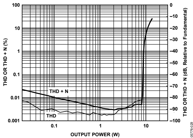
Figure 29. THD and THD + N vs. Output Power, 1 kHz Sine, 6 \Omega Load, PVDD = 18 V
