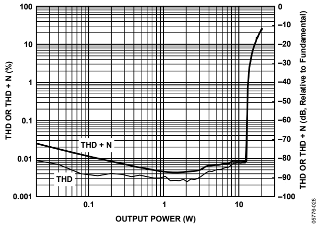
Figure 28. THD and THD + N vs. Output Power, 1 kHz Sine, 4 \Omega Load, PVDD = 18 V
