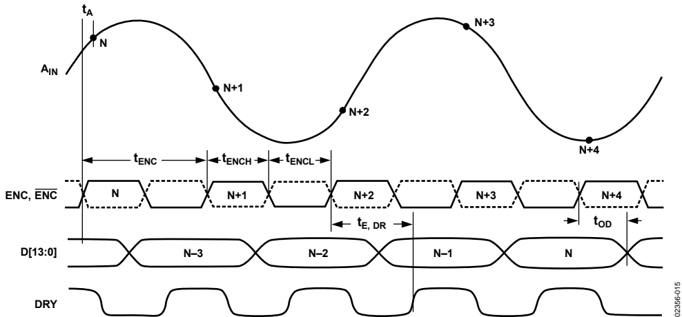
Figure 2. Timing Diagram
