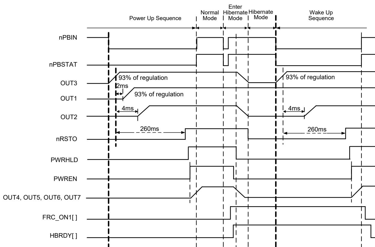
Figure 5: Hibernate Mode Sequence ACT8892Q4I134-T
