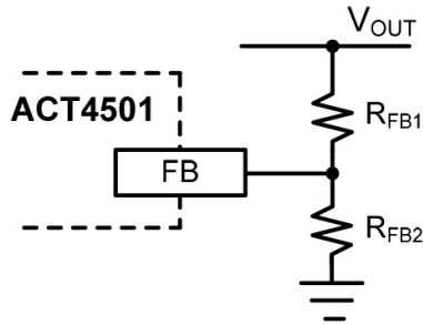
Output Voltage Setting
