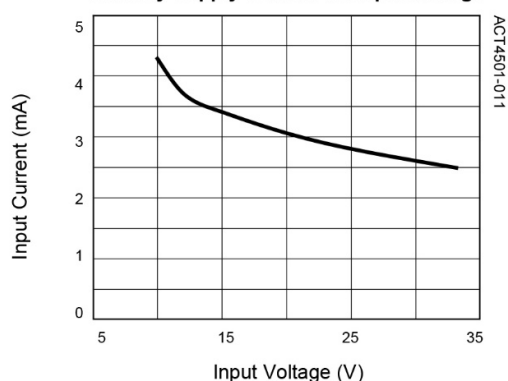
Standby Supply Current vs. Input Voltage
