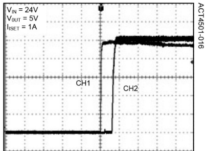
Start up with EN
