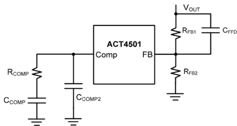
Frequency Compensation for High RFB1
