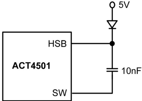
Figure 3: External High Voltage Bias Diode
