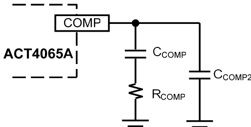
Stability Compensation
