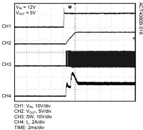
Start Up with V_{\text{IN}} (Load 2A)
