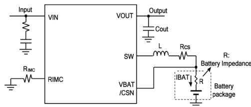
Figure 10. Battery impedance compensation setting circuit
