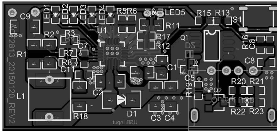
Figure 15. PCB Layout
