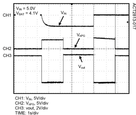
Transition Between Buck Mode and Boost Mode
