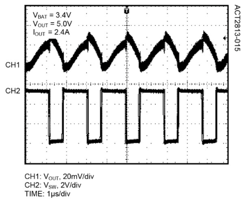
SW and Output Waveforms in Boost Mode
