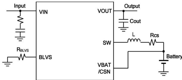
Figure 4: Battery level voltage shift setting current
