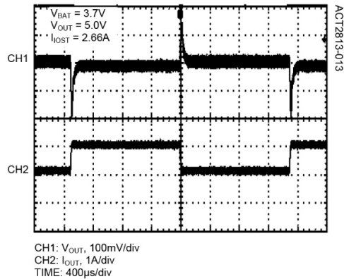
Boost Load Transient (80mA-1A-80mA)
