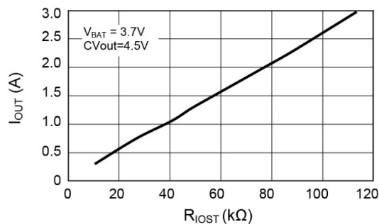
Figure 8. Boost Output current setting
