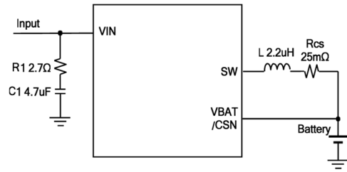
Figure 13. Input over voltage surge protection circuit
