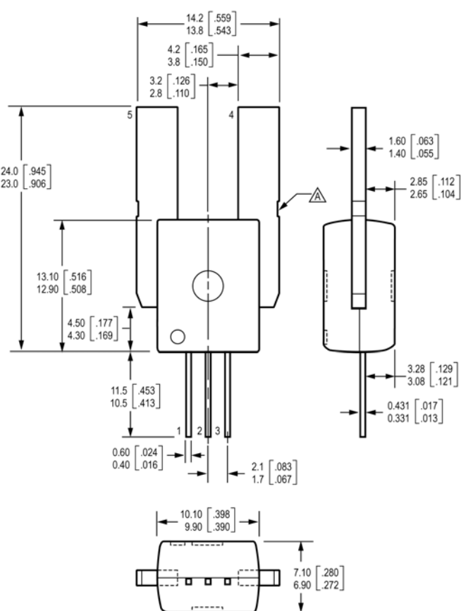
Package CB-PSS
