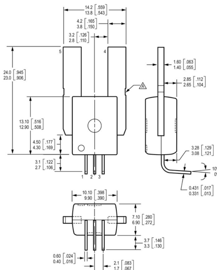
Package CB-PSF
