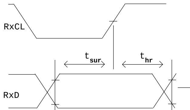
Receive set-up and hold times
