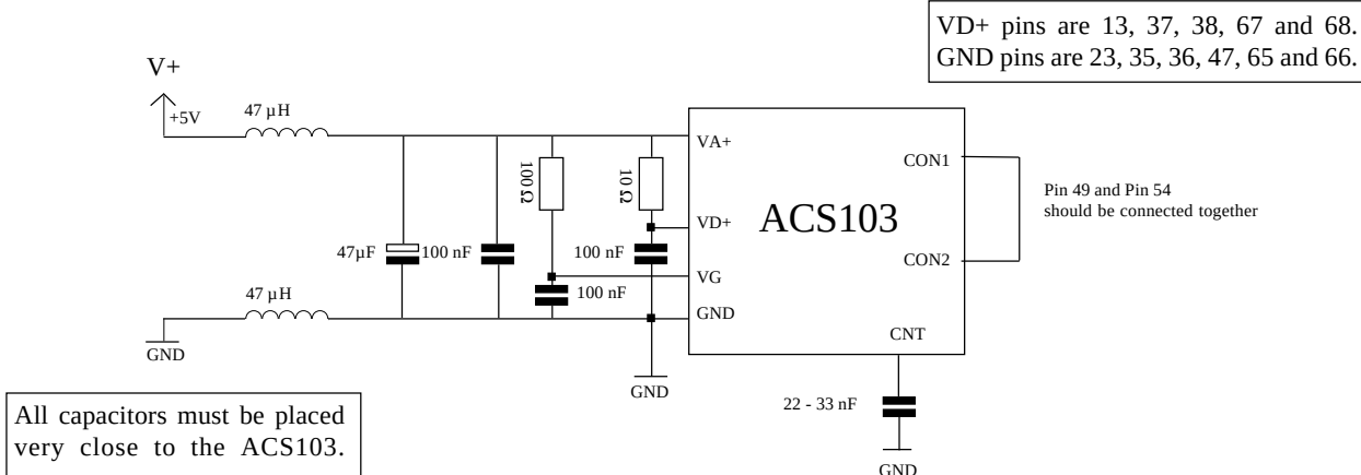
Figure 3. Recommended power supply layout
