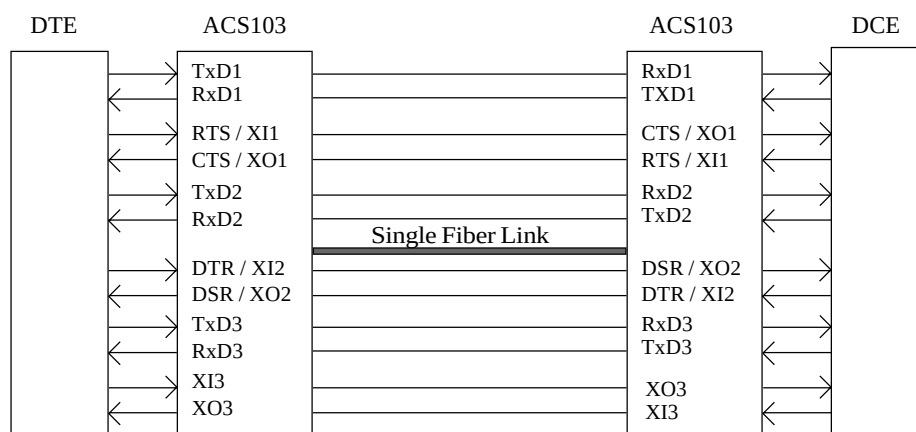
Figure 4. 6 Full-duplex channels in data transmission mode
