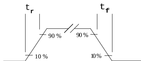
Digital Outputs rise and fall times
