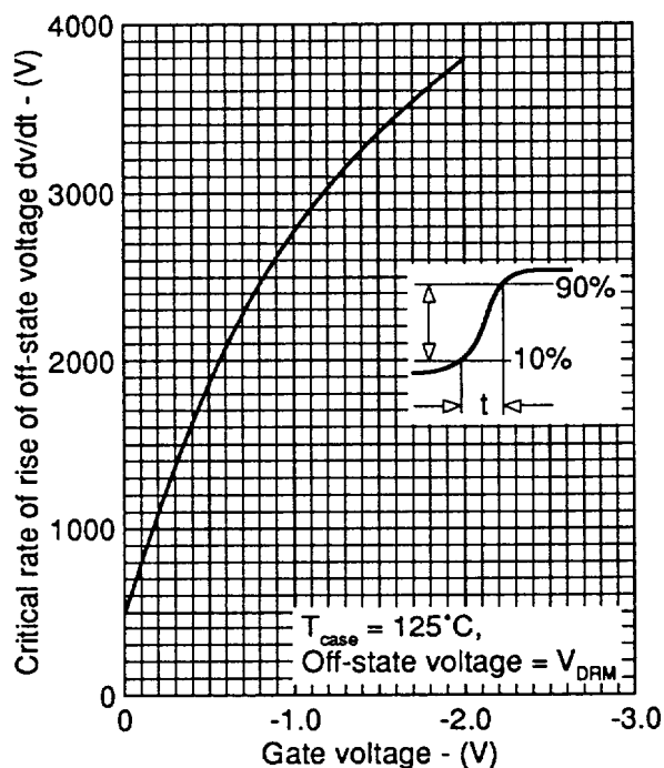
FIG. 7 MINIMUM LINEAR CRITICAL RATE OF RISE OF OFF-STATE VOLTAGE vs GATE VOLTAGE
