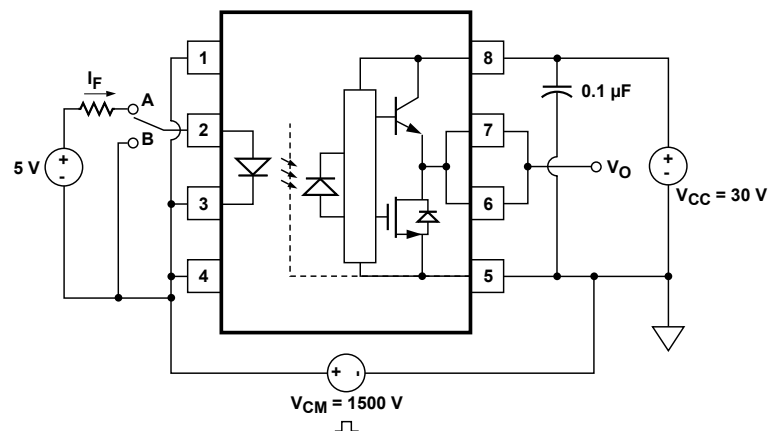
Figure 22. CMR test circuit and waveforms.
