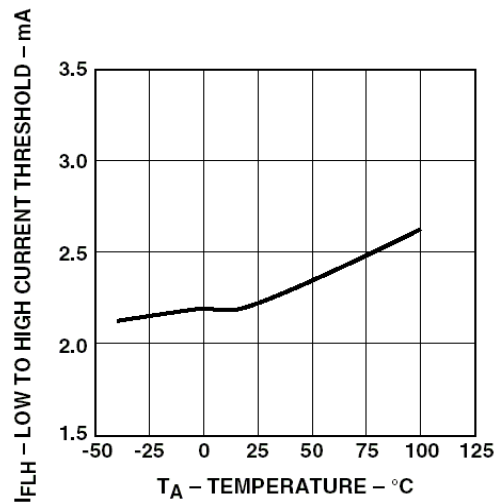
Figure 9. I_{FLH} vs. Temperature.
