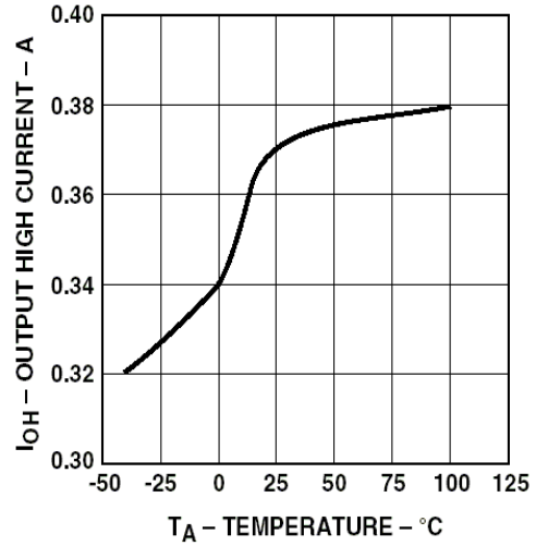
Figure 2. I_{OH} vs. Temperature.
