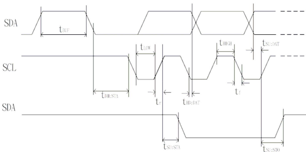
I2C interface
