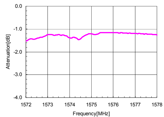
Figure 26. Ant-GPS Insertion Loss.
