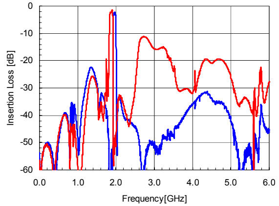
Figure 10. PCS Tx-Ant and Rx-Ant Wideband Insertion Loss.
