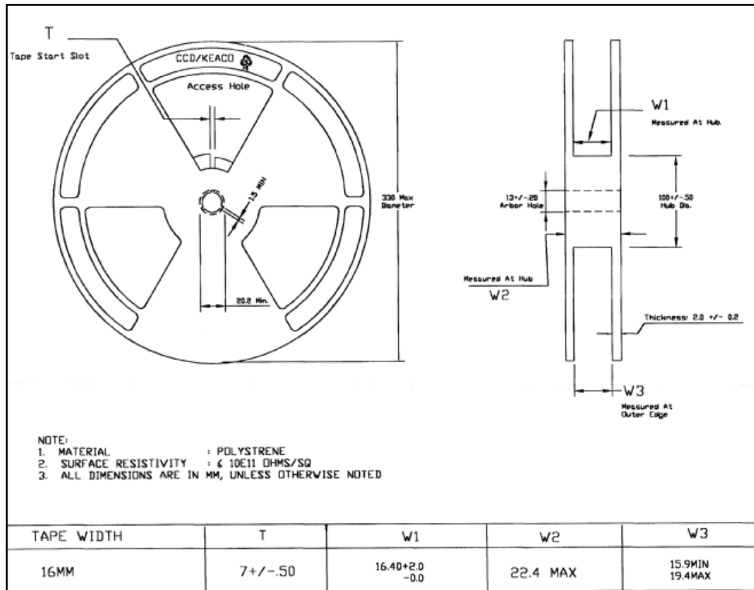
Figure 38. Reel Information.
