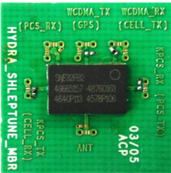
Figure 2. Test Circuit with ACFM-7101 Quintplexer.
