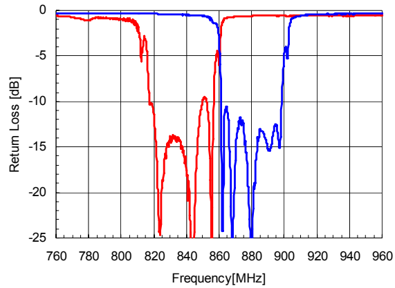
Figure 15. Cellular Tx and Rx Return Loss.
