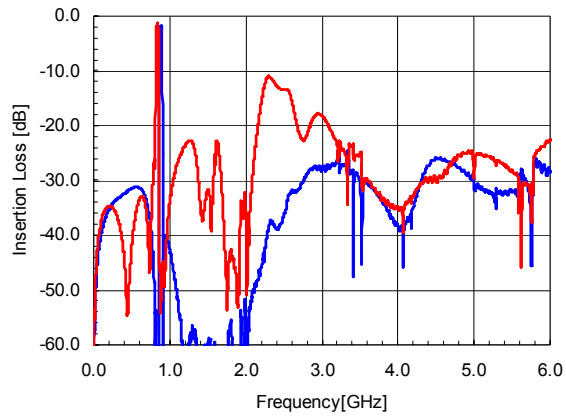
Figure 21. Cellular Tx-Ant and Ant-Rx Wideband Insertion Loss.
