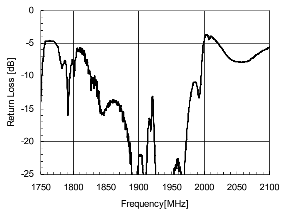
Figure 8. PCS Antenna Port Return Loss.
