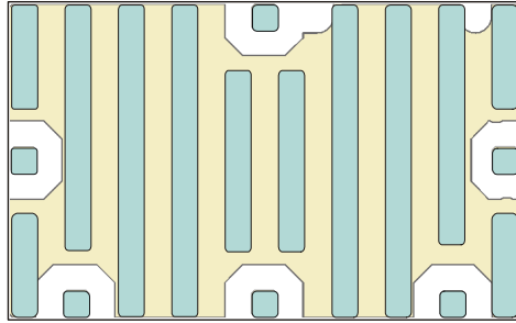
Figure 33. Solder Stencil Overlayed on ACFM-7101 Bottom Metal Pattern.
