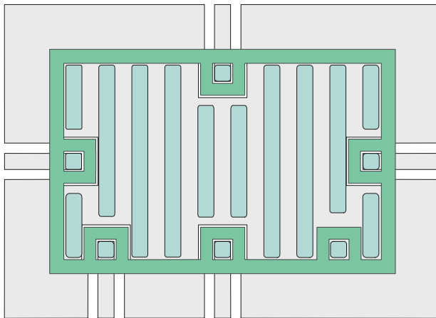
Figure 34. Solder Stencil and Solder Mask Overlayed on Land Print.
