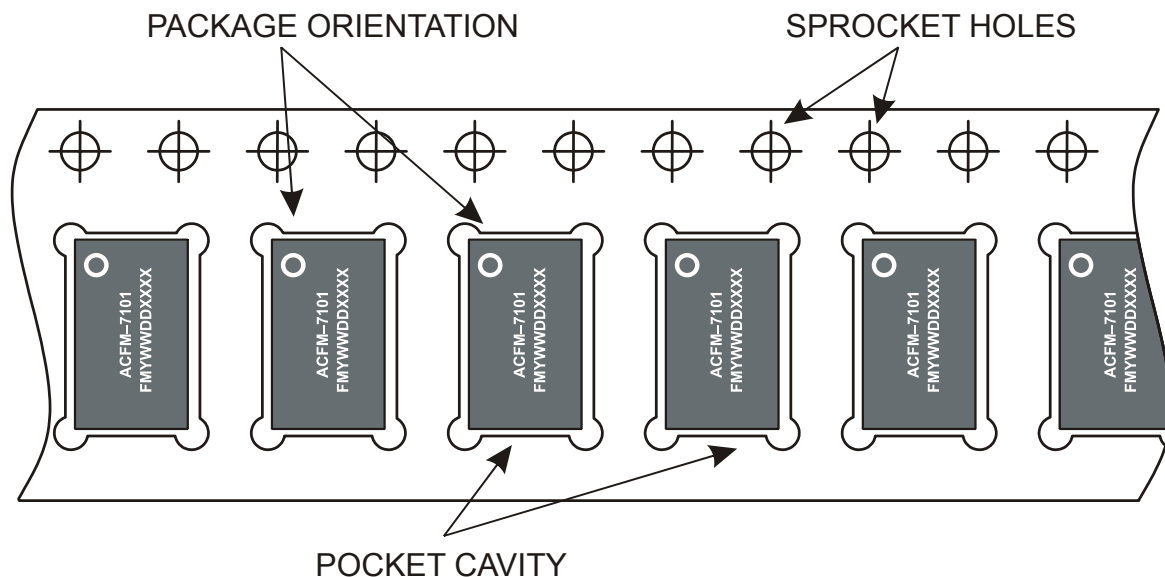
Figure 37. Orientation in Tape.
