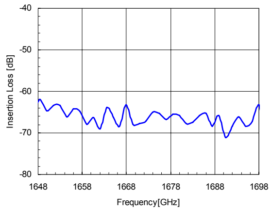
Figure 22. Cellular Ant-Rx Rejection at Tx Second Harmonic.
