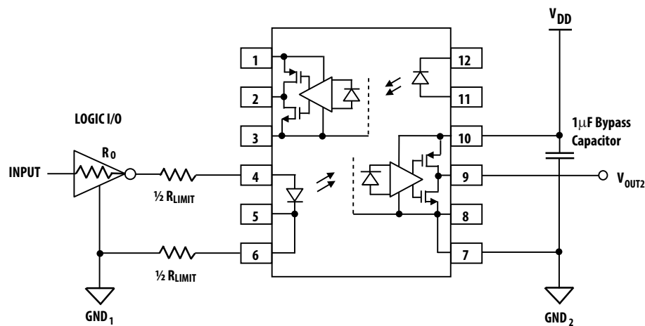
Figure 12. Recommended Application Circuit for ACFL-6212T Low Power Performance
