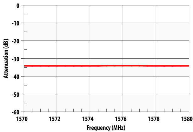
Figure 6. Rejection in GPS Band
