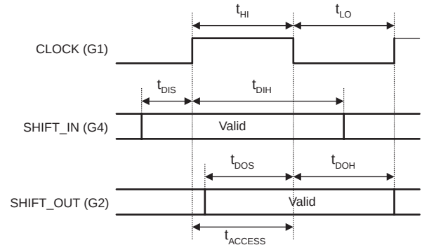
Figure 31. Serial Data Timing
