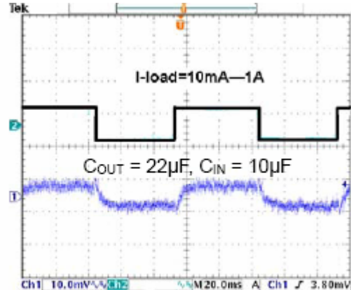
Load Transients
