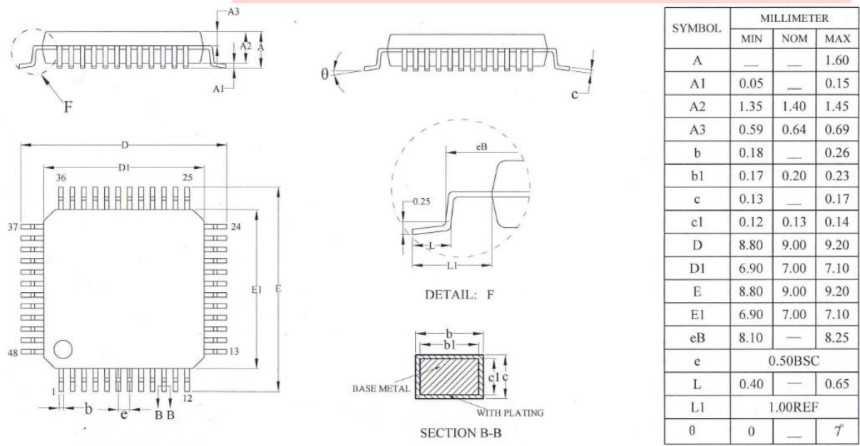
Figure 3-1. AC6921A_LQFP48 Package
