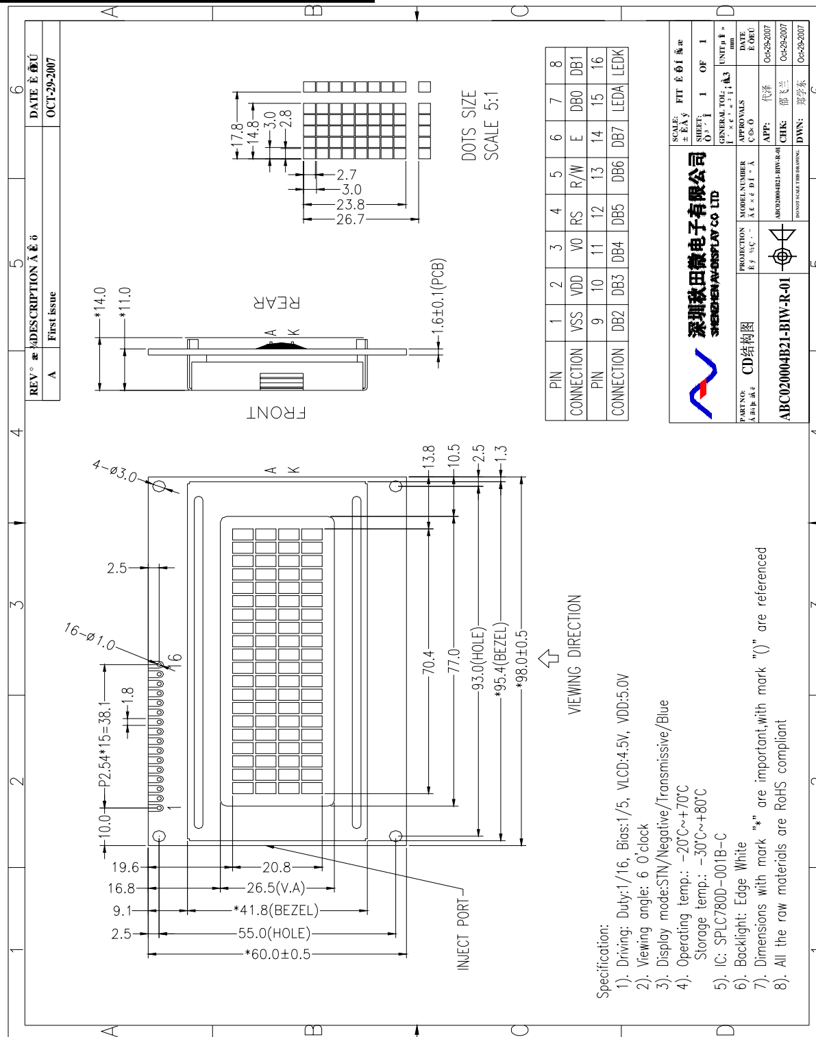
Figure 1. Dimensional outline
