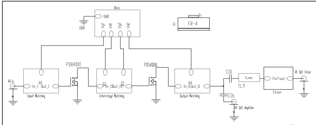
Figure 12. Circuit schematic
