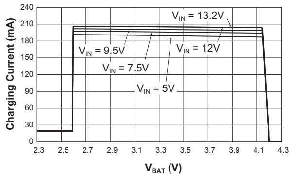
www.datasheet4u.com Constant Charging Current vs. V_{BAT} ( R_{SET} = 8.87k\Omega )
