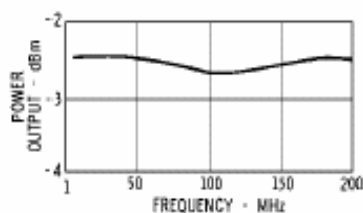
Power Output*
