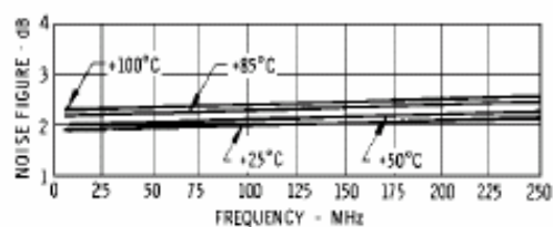
Noise Figure
