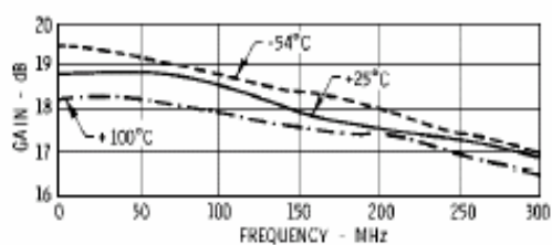
Gain
