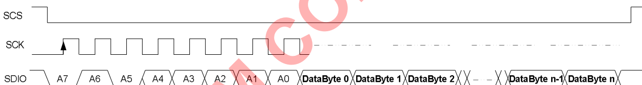
Figure 10.10 TX FIFO Write Command
