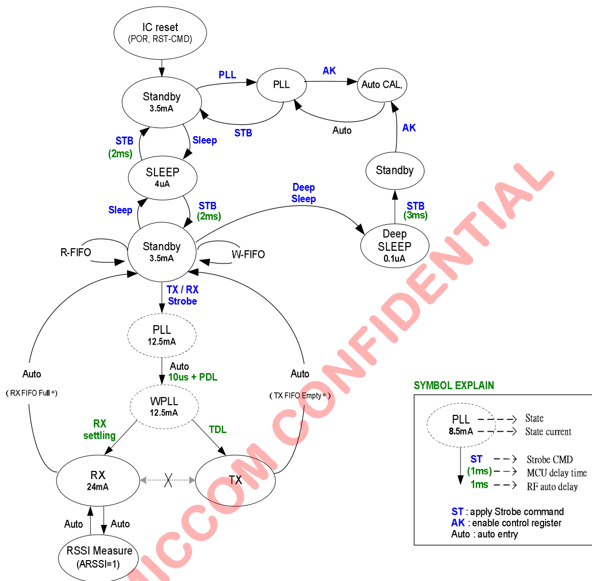
Figure 11.3 State diagram of FIFO Mode
