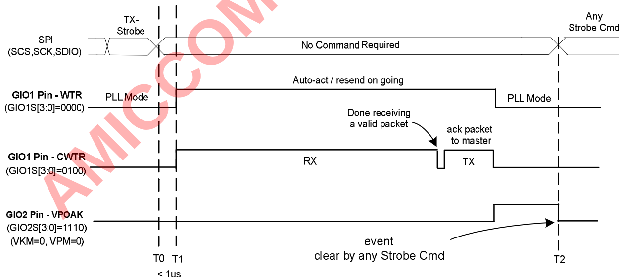
The receiver site (auto-ack)
