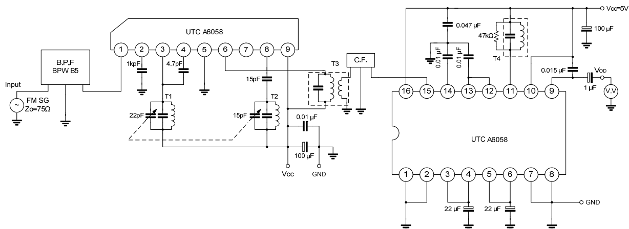
Test Circuit 2
