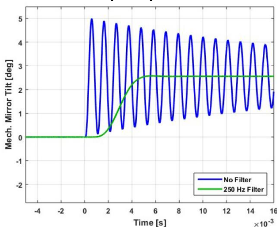
Step Response
