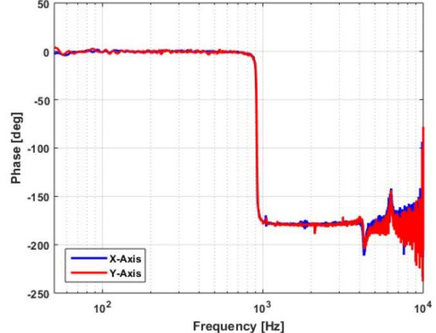
Small Signal Frequency Response - Phase
