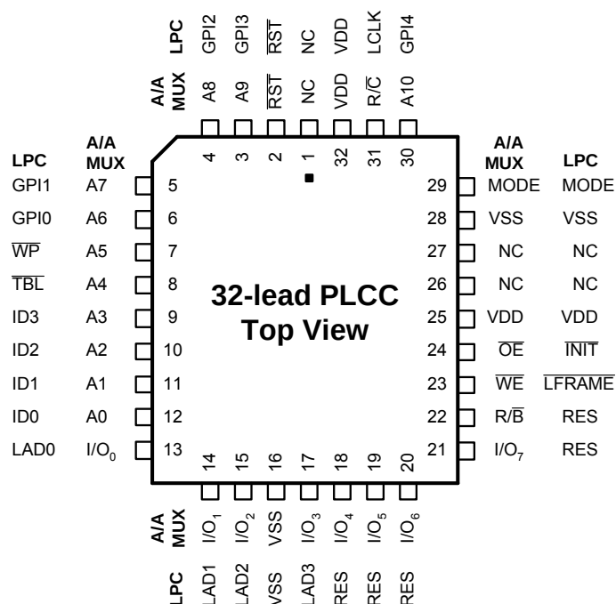
Figure 1: Pin Assignments for 32-Lead PLCC
