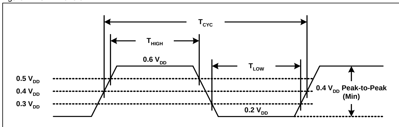
Figure 4: LCLK Waveform
