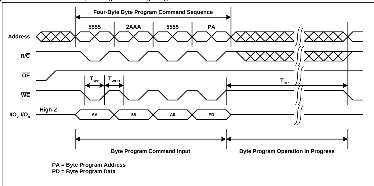
Figure 14: A/A Mux Mode Byte Program Timing Diagram
