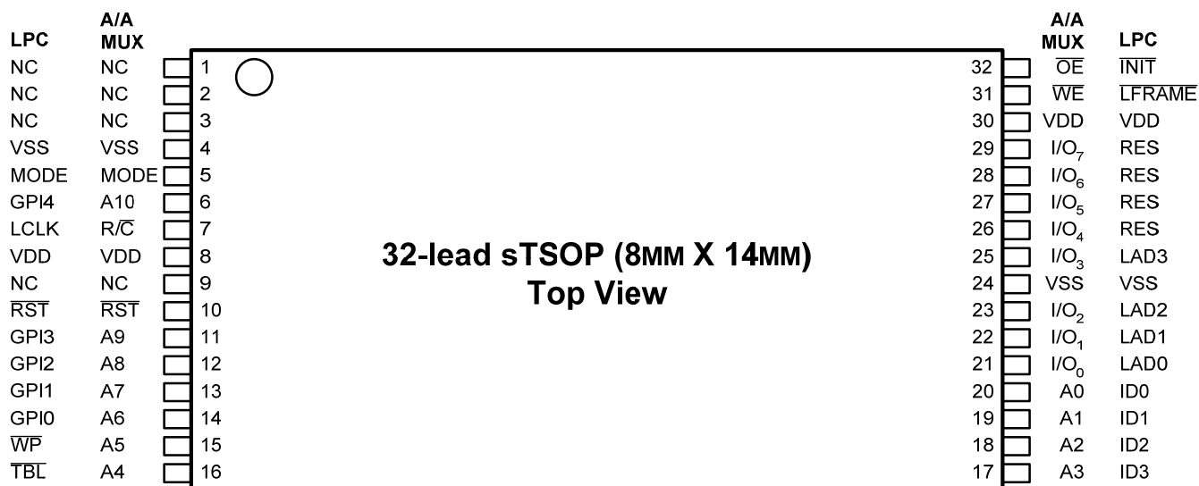
Figure 2: Pin Assignments for 32-Lead sTSOP
