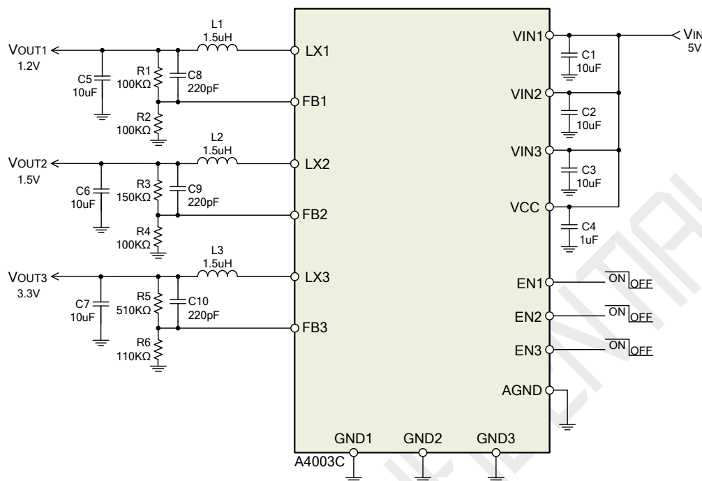
Figure 1. Typical application circuit diagram
