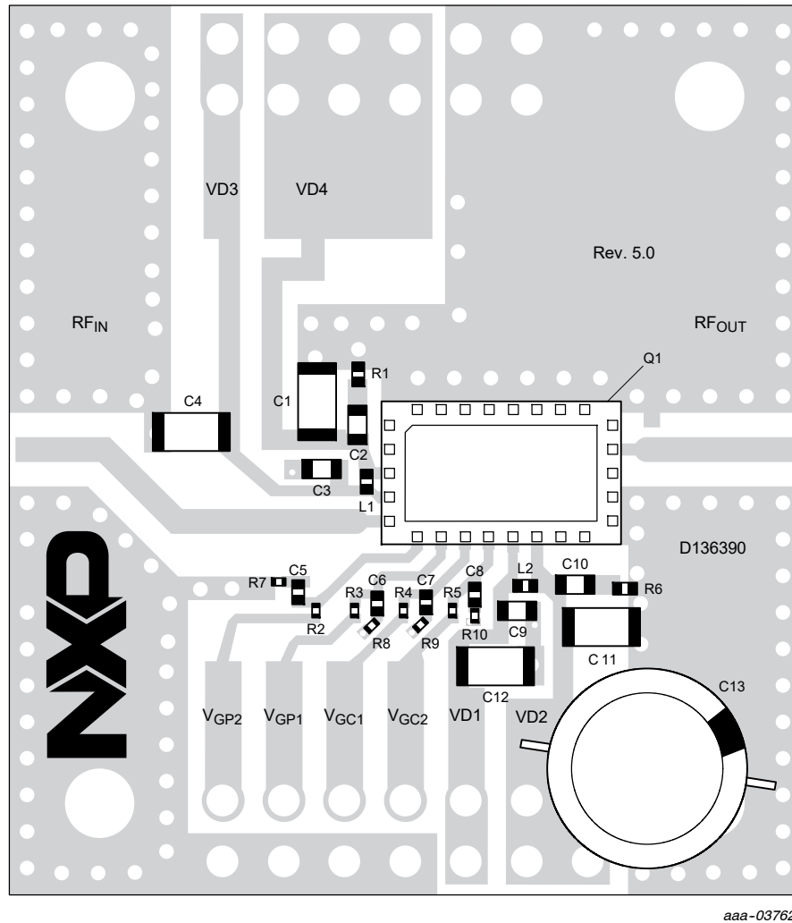
Figure 2. A3M39TL039 Reference Circuit Component Layout
