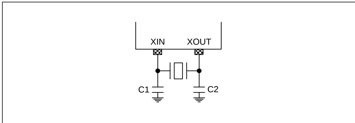
Figure 59. Crystal/Ceramic Oscillator
