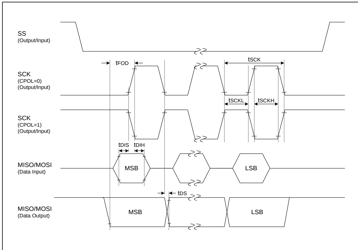
Figure 55. SPI Timing
