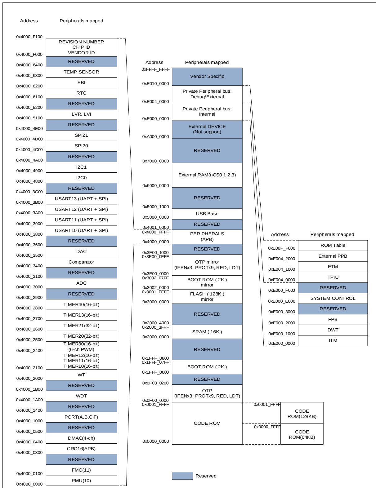
Figure 6. Memory Map
