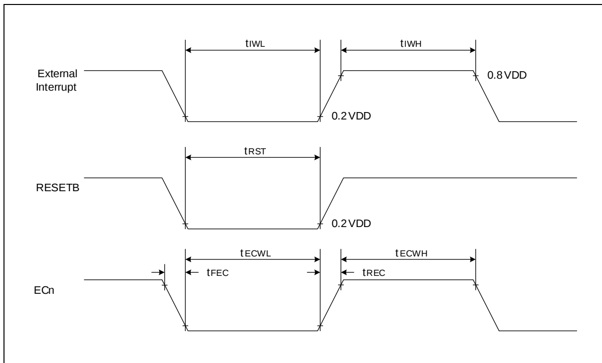
Figure 54. AC Timing
