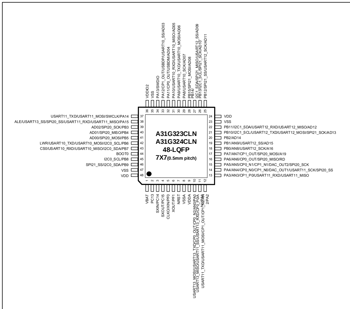
Figure 3. LQFP 48 Pinouts
