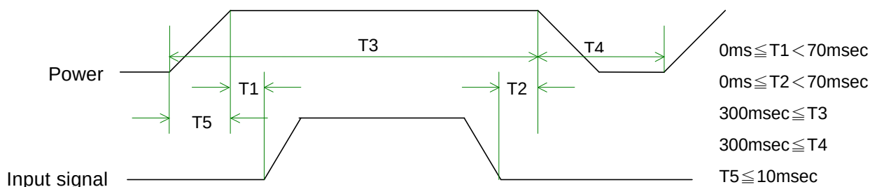
Sequence of Power-on/off and signal-on/off
