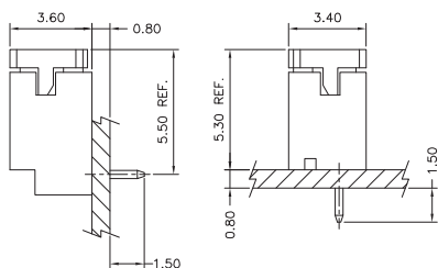
DIP TYPE
