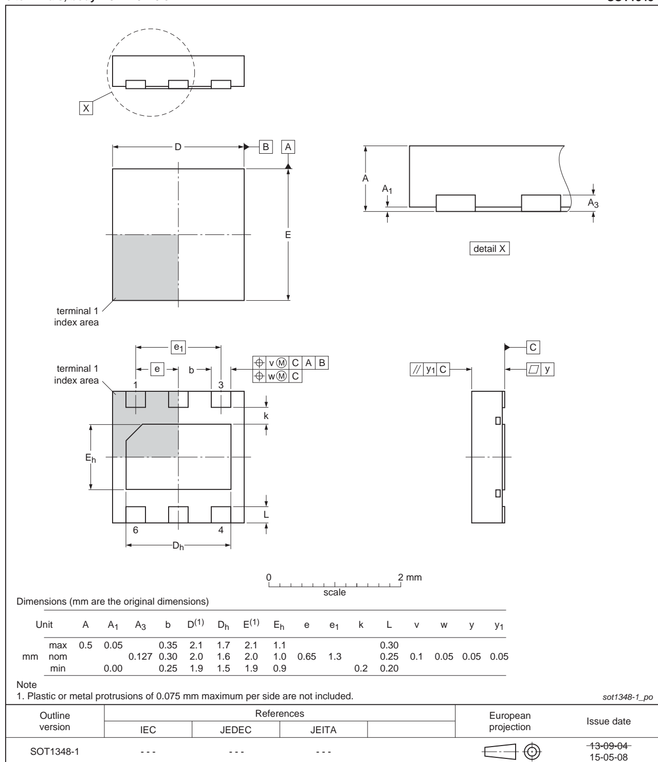
Fig 7. Package outline SOT1348-1 (HXSON6)
