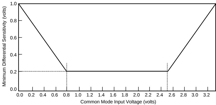
Figure 45. Differential Input Sensitivity Over Entire Common Mode Range
