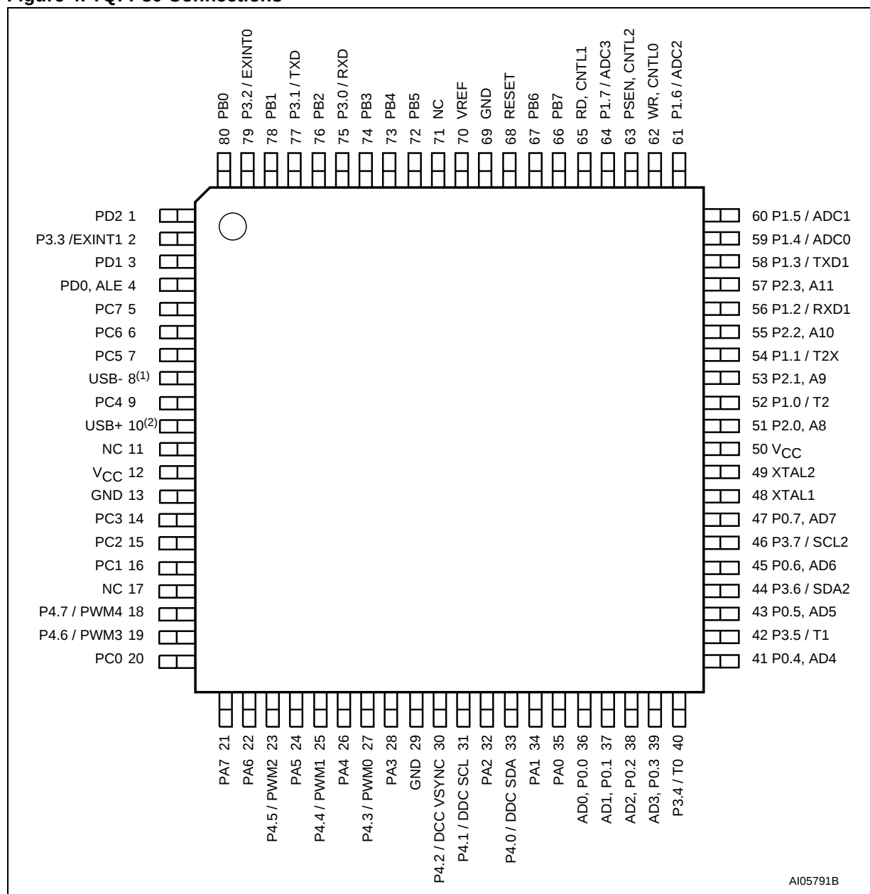
Figure 4. TQFP80 Connections
