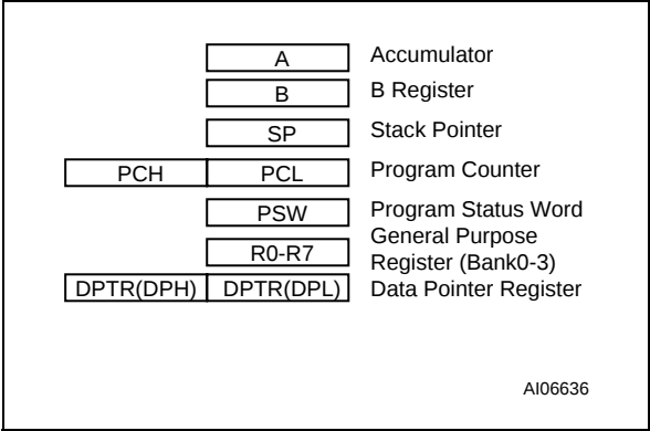
Figure 6. 8032 MCU Registers
