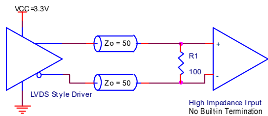
Figure 17. LVDS Termination
