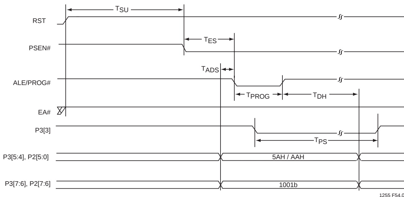
FIGURE 14-22: Prog-SC0 / Prog-SC1
