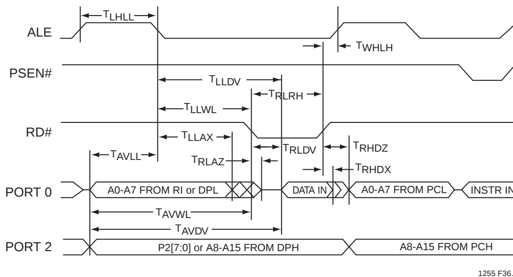
FIGURE 14-4: EXTERNAL DATA MEMORY READ CYCLE
