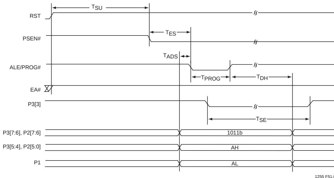
FIGURE 14-19: SECTOR-ERASE
